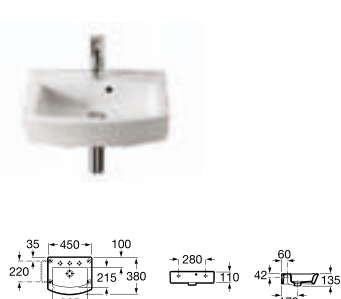
挂墙洗脸盆 327624..0 (450x380)
