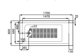
Tampa 坦帕 2N0860..0 (1700x800mm)
