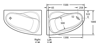
Waitara 威泰角形 247263..1 /247259..0 左裙 (1500x1000mm) 247264..1 /247260..0 右裙 (1500x1000mm)
