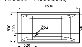
Vythos 韦德 26N004..0 (1600x800mm) 26N005..0 (1600x800mm)
