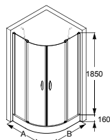
Corner 圆弧形淋浴房(2固2活) N10100112 中间开门 (1000x1000mm) N10100212 中间开门 (900x900mm) N10100312 中间开门 (800x800mm)
