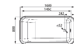
Element 伊元素独立式 26N001..0 (1600x800mm) / 26N002..0 可带缸边浴缸龙头 26N003..0
