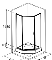
Diamond 钻石型淋浴房(2固1活) N102L0112 / N102R0112 左开门/右开门 (1000x1000mm) N102L0212 / N102R0212 左开门/右开门 (900x900mm)
