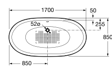
Newcast Drop in 纽凯 233650..0 无裙 (1700x850mm)
