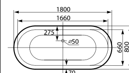
Ibiza 艾比莎 26N008..0 (1800x800mm)
