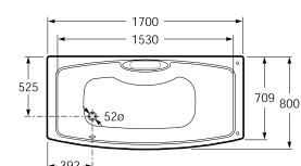
Dama senso 丹圣 247607..1 /247606..0 (1700x800mm)
