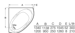
Genova corner 杰诺娃角形 247420..1 /247416..0 (1340x1340mm) 247421..1 /247417..0 (1200x1200mm)
