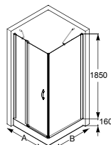
Rectangle 长方形淋浴房(2固1活) N103L0412 左开门 (1000x800mm) N103R0412 右开门 (1000x800mm)
